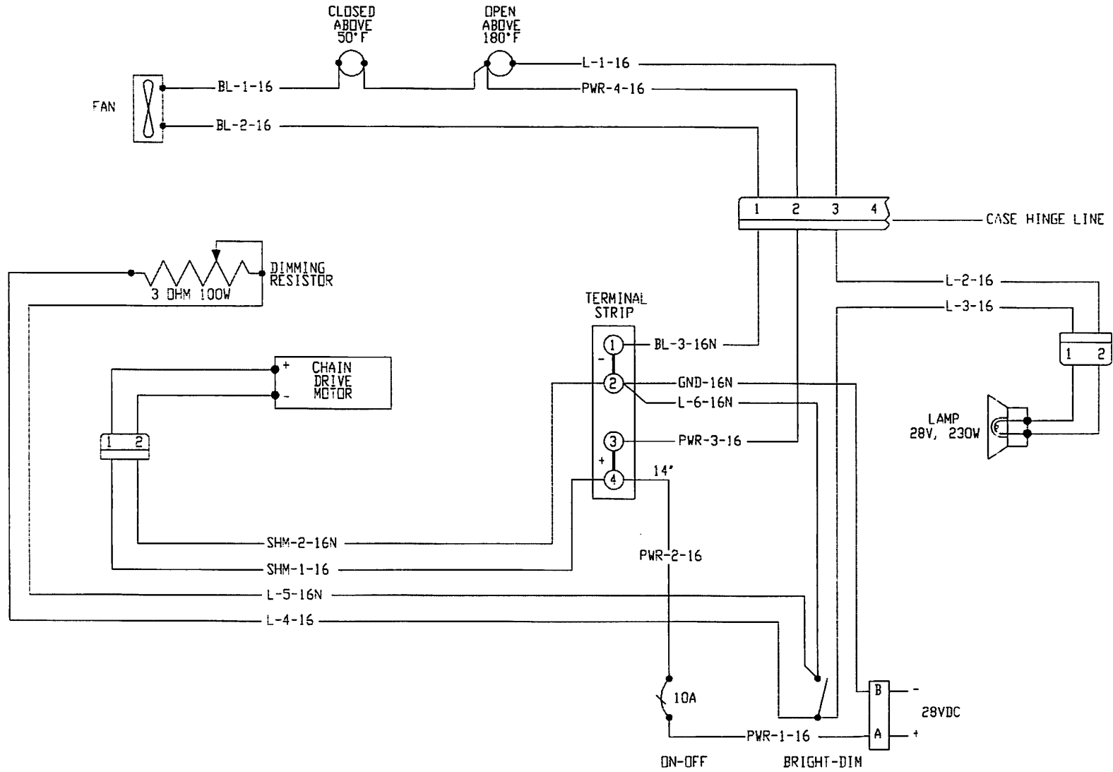
Figure 1 28 VDC MINI-PLASI Wiring Diagram
